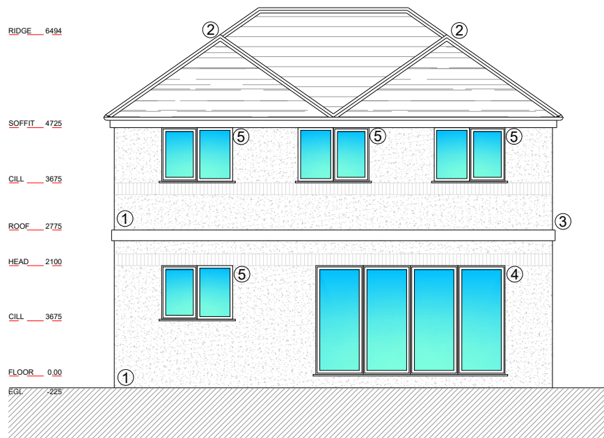
REAR ELEVATION
